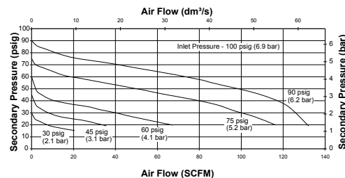
3/8" 1500 SERIES F-R-L COMBO
