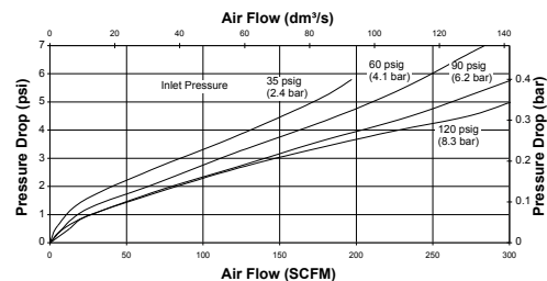
3/4" 3000 SERIES LUBRICATOR
